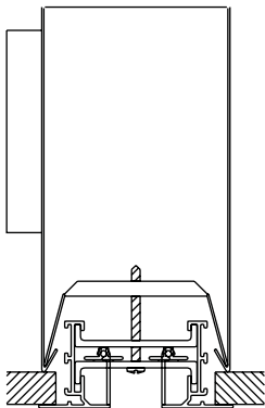
FlowBar Border Type 77 Installation detail
